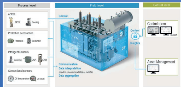
Concept of an intelligent transformer with ETOS®
